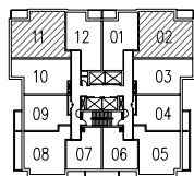
KEYPLAN 21st FLOOR PLAN
