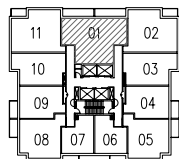
KEYPLAN 24th-28th FLOOR PLAN
