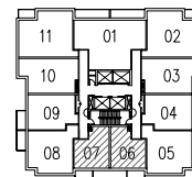
KEYPLAN 24th–28th FLOOR PLAN
